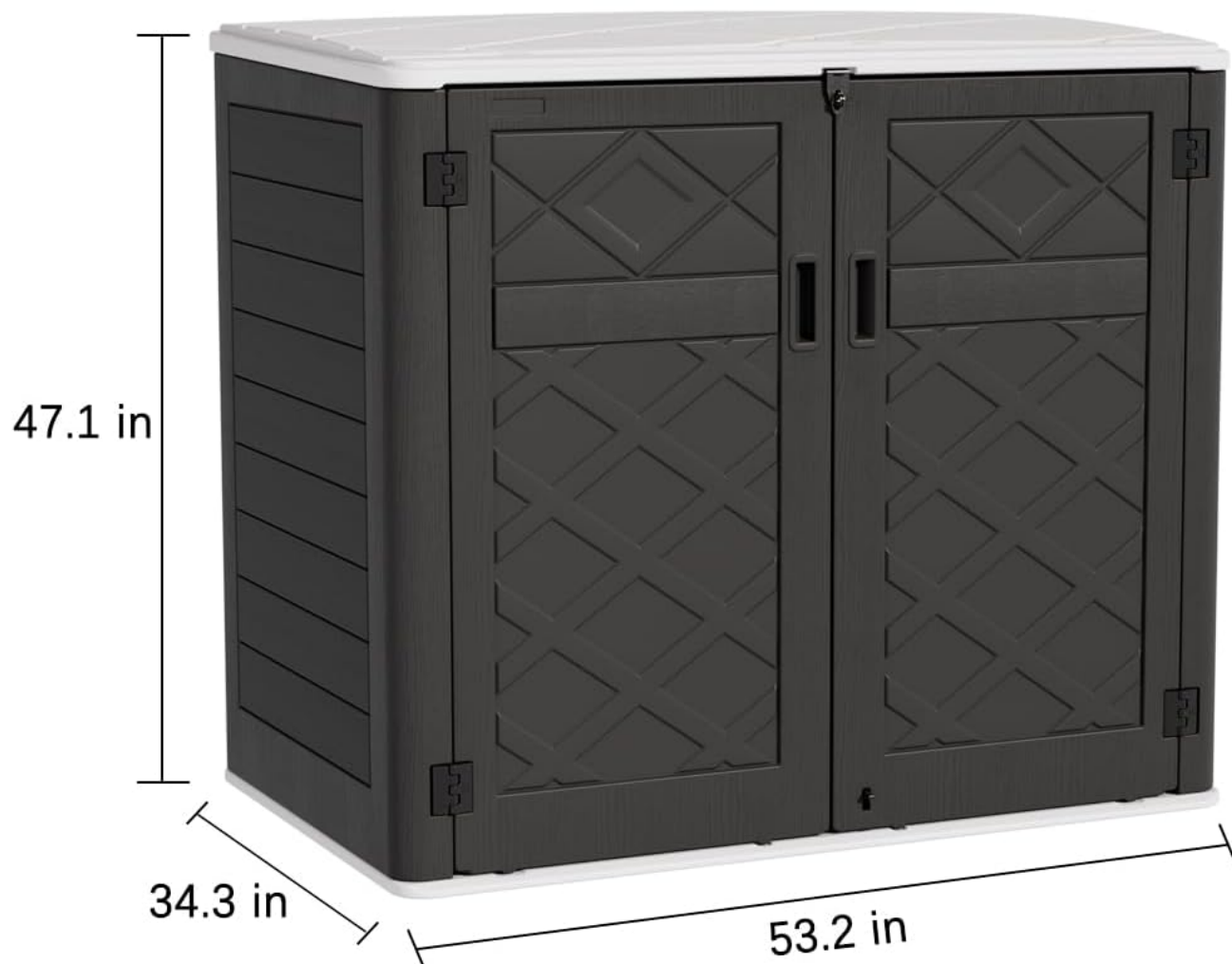
Figure 2: Product Dimensions (External: 53.2"W x 34.3"D x 47.1"H; Internal: 50"W x 30.1"D x 43"H)
