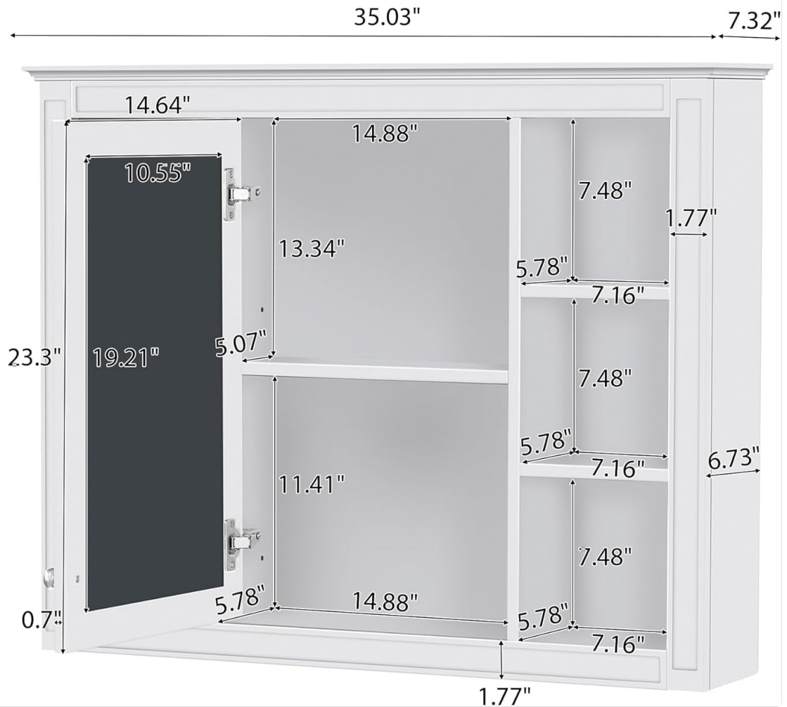
Figure 4: Cabinet dimensions for planning installation.
