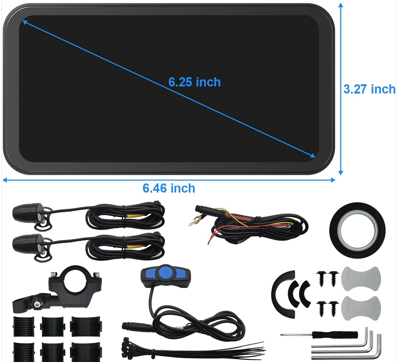
Figure 2: Detailed view of the packing list, illustrating the main unit, cameras, remote, and various installation accessories.
