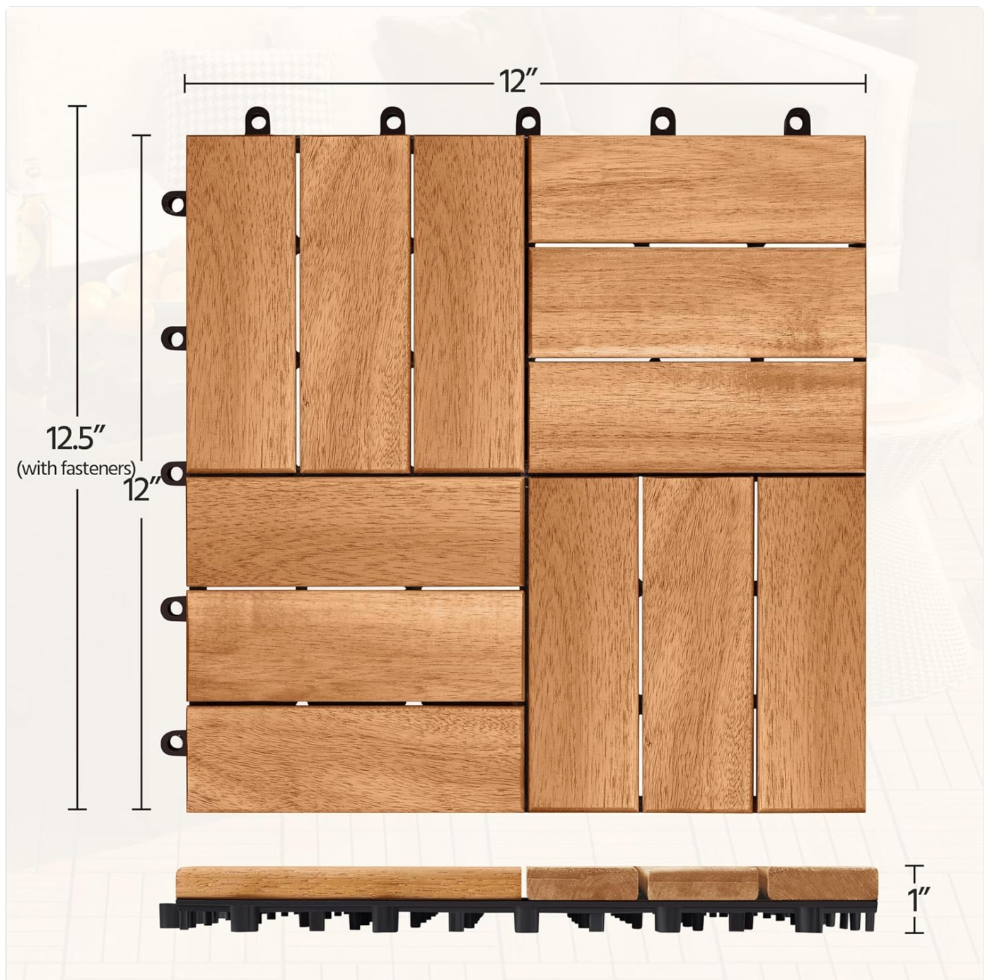
Image: Dimensional specifications of the deck tiles.
