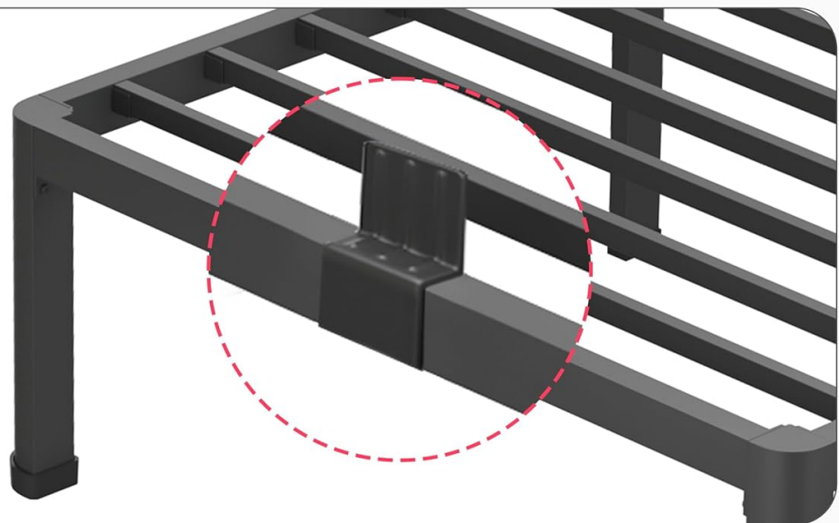
Figure 4: Correct installation of mattress stoppers to prevent mattress sliding.
