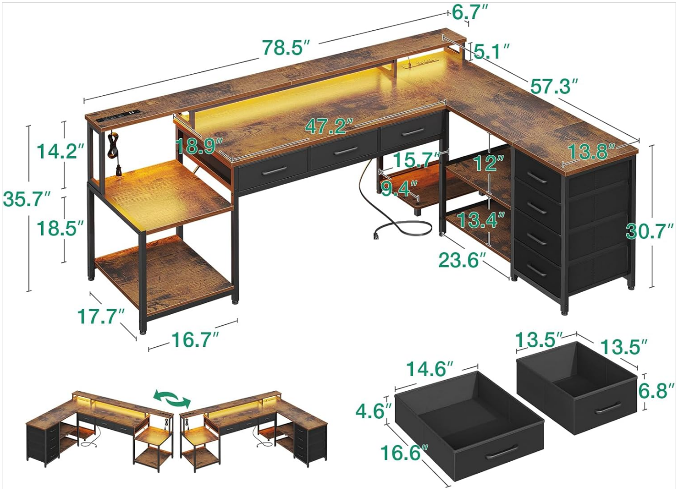
Image 4.1: Desk dimensions and illustration of the reversible design.
