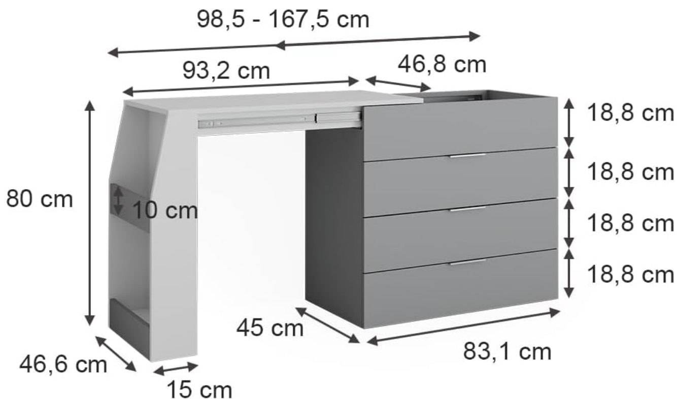
Image 8.1: Technical drawing showing the detailed dimensions of the Vicco Iva Craft Table in both compact and extended states.
