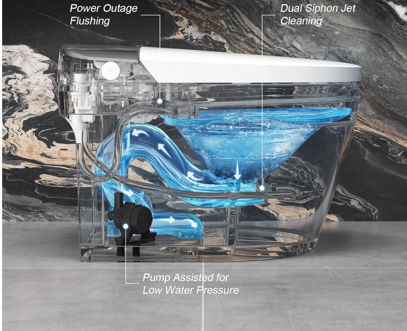
Figure 8: Internal mechanism for pump-assisted powerful flush.
