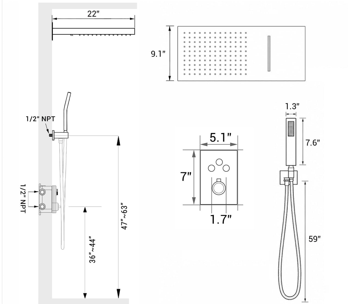
Image 6.1: Dimensional specifications of the shower system components.
