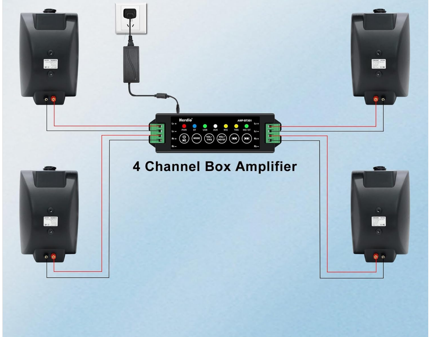
Image: A clear diagram illustrating the wiring connections between the four speakers and the 4-channel amplifier.
