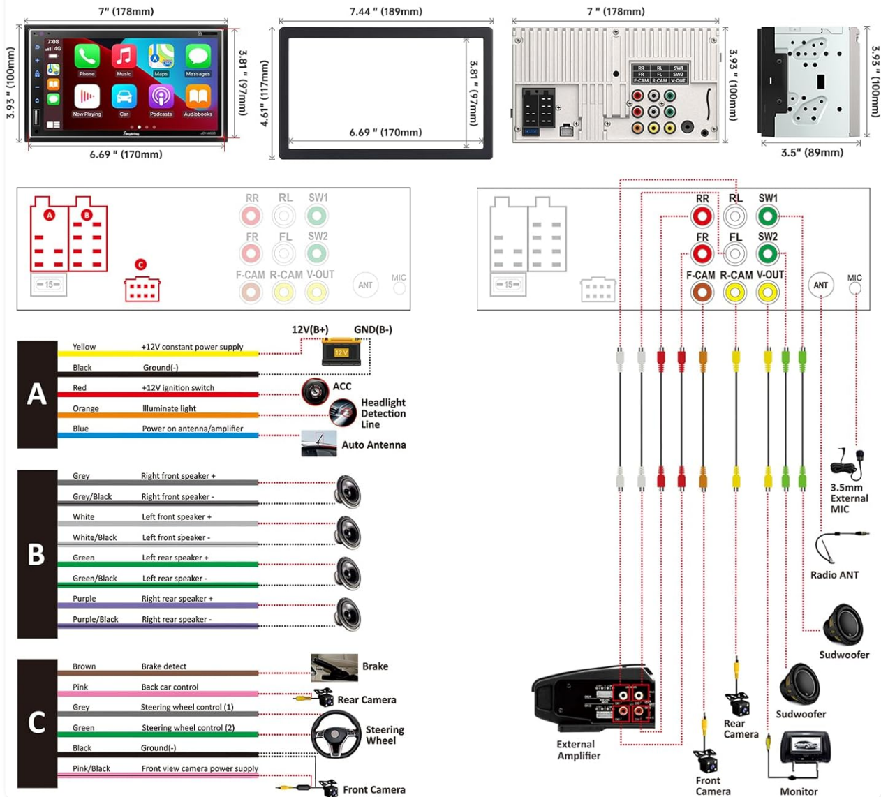
Image: Comprehensive ISO standard double DIN size diagram with detailed wiring connections for power, speakers, cameras, and other accessories.
