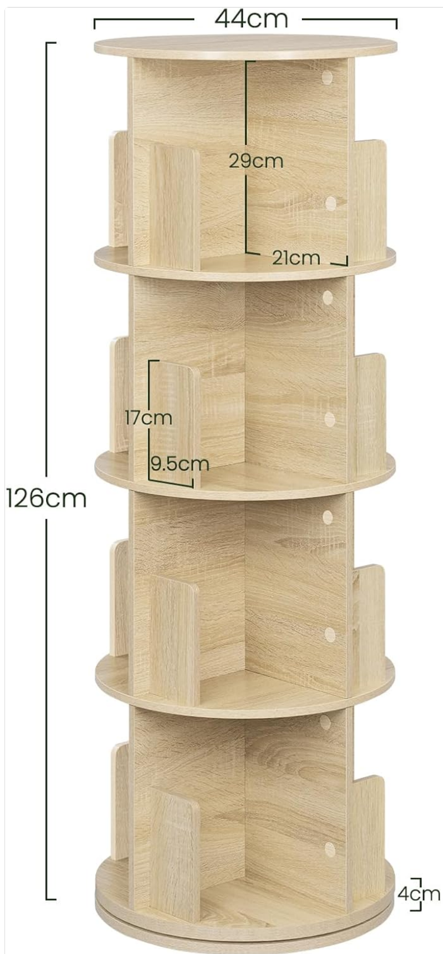
Image 8.1: Detailed dimensions of the 4-tier rotating bookshelf.
