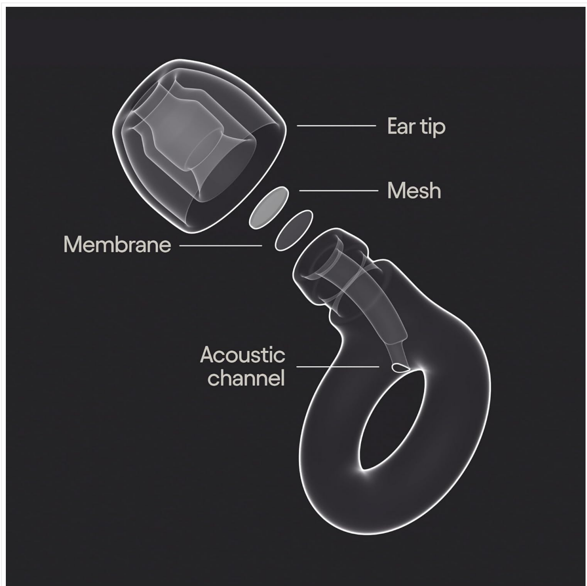
Figure 4.1: Exploded view illustrating the acoustic channel, mesh filter, membrane, and ear tip components of the Loop Experience 2 Ear Plugs.
