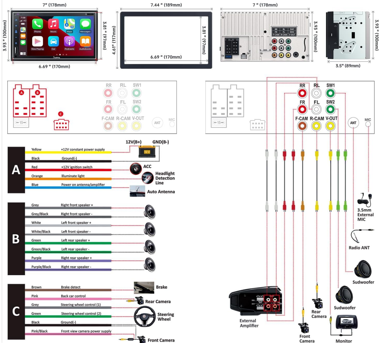
Image 3.1: ISO Standard Double DIN wiring and dimension diagram.
