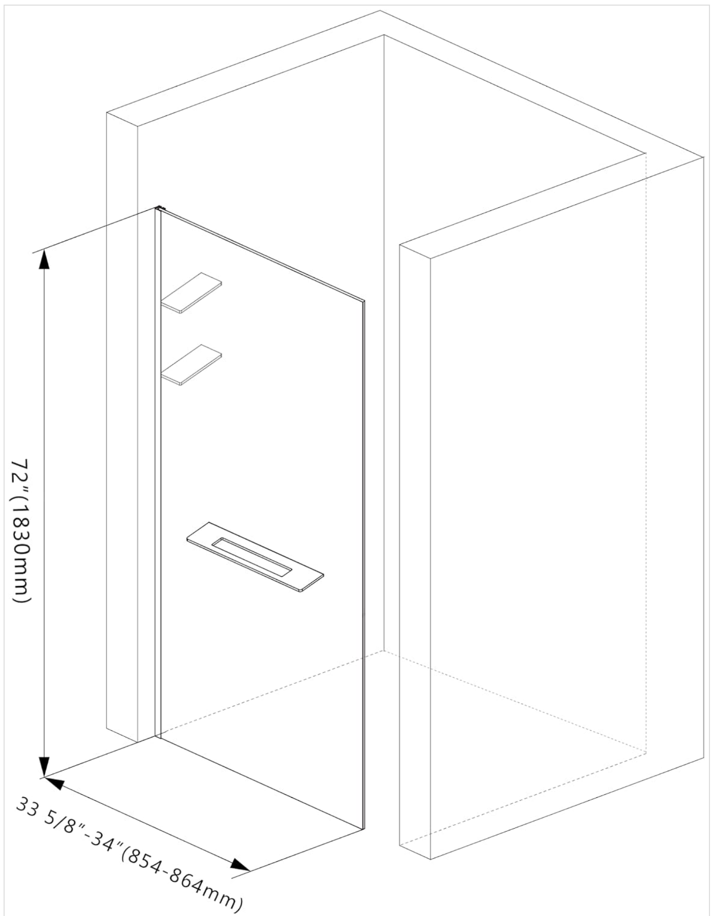
Figure 3.2.1: Shower Panel Dimensions
