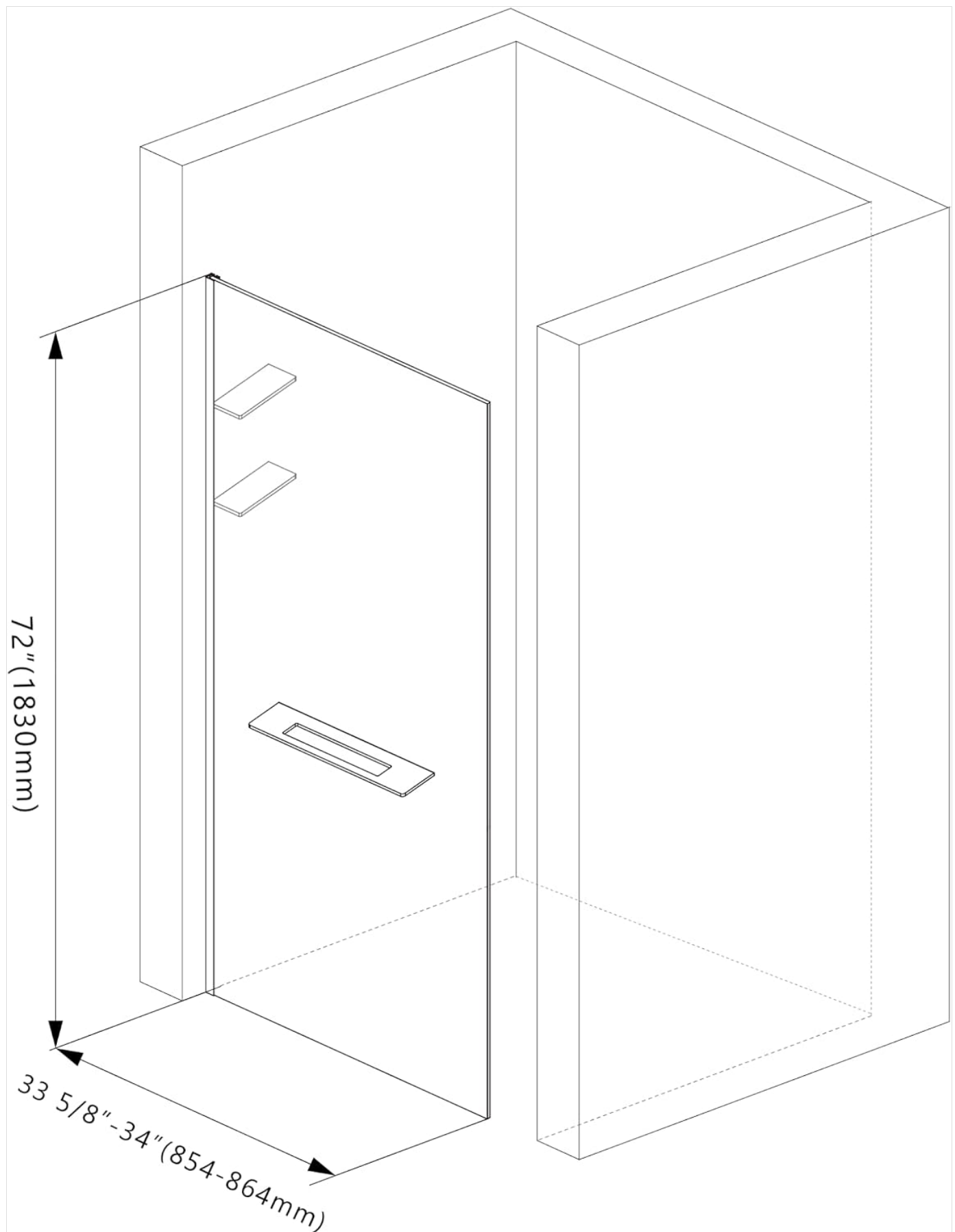
Image: Detailed diagram illustrating the dimensions of the shower panel (33 5/8" - 34" width, 72" height) and the recommended 10mm gap for the wall profile.
