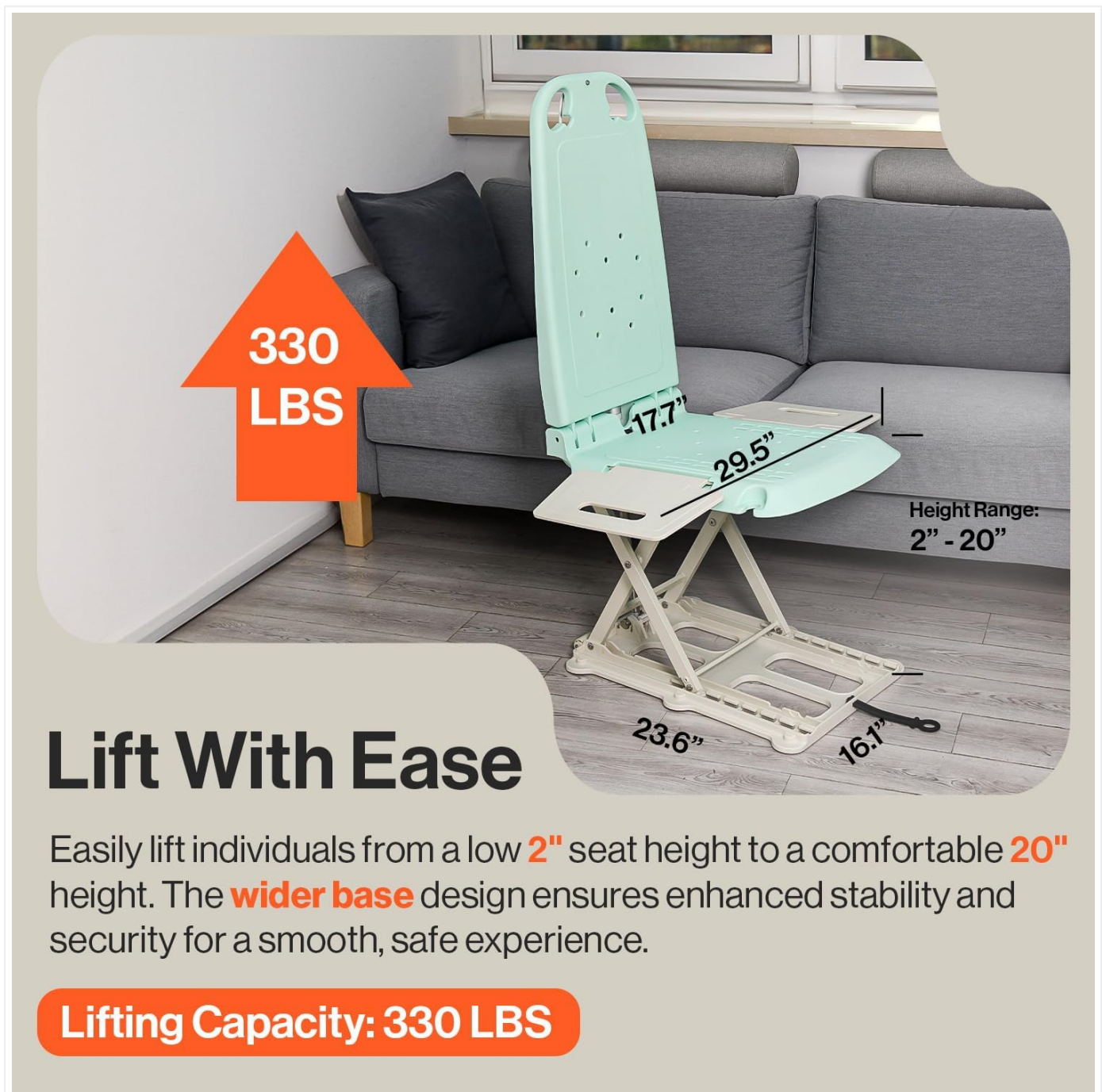
Figure 3: Lift capacity and dimensions.
