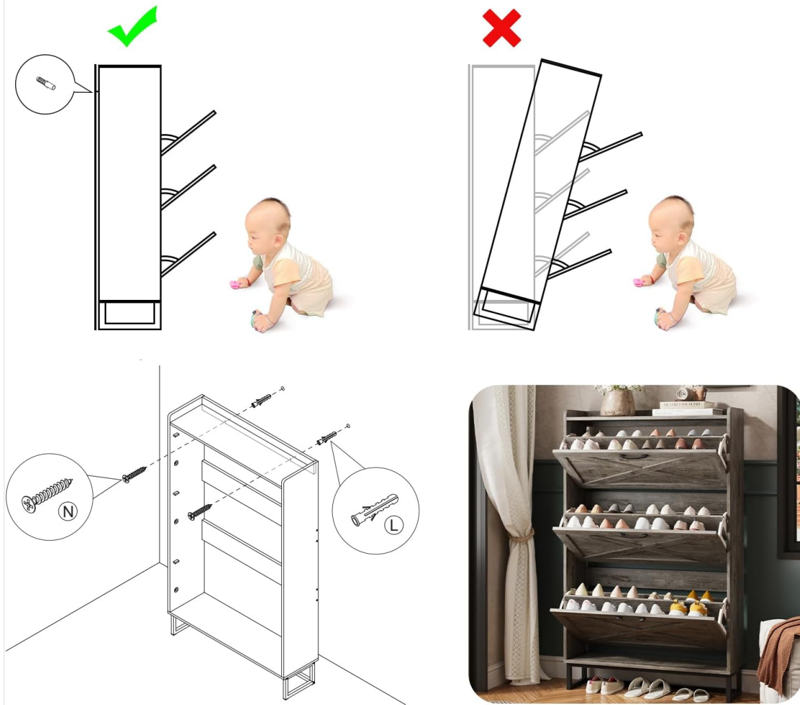
Image: Illustration of the anti-tipping device installation, showing how to secure the cabinet to the wall to prevent accidents.
