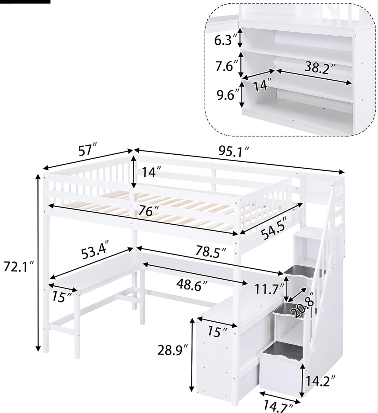
Image 2.1: Product dimensions for the Merax Full Size Loft Bed Frame.
