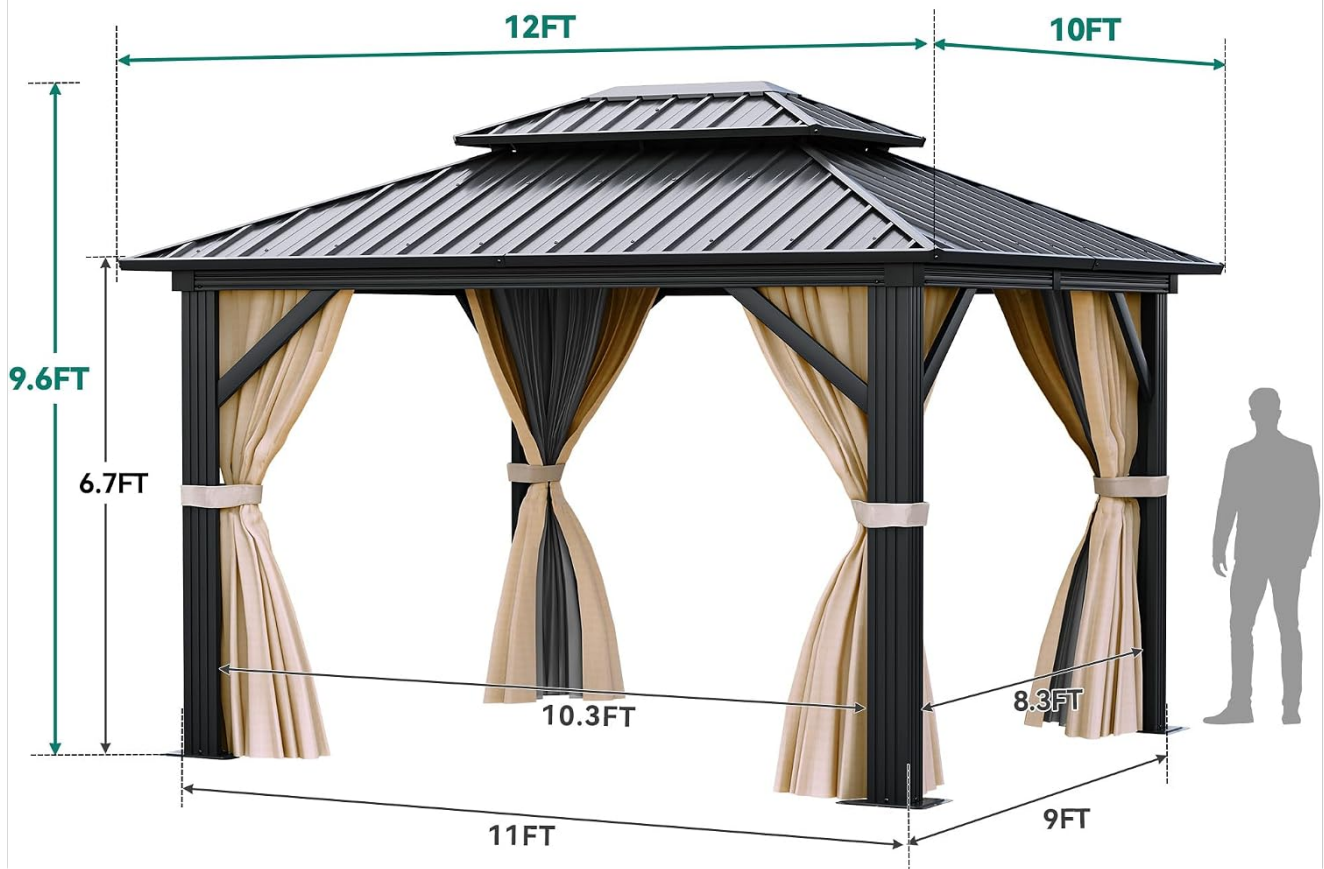
Image: Detailed dimensions of the YITAHOME 10x12ft Gazebo.
