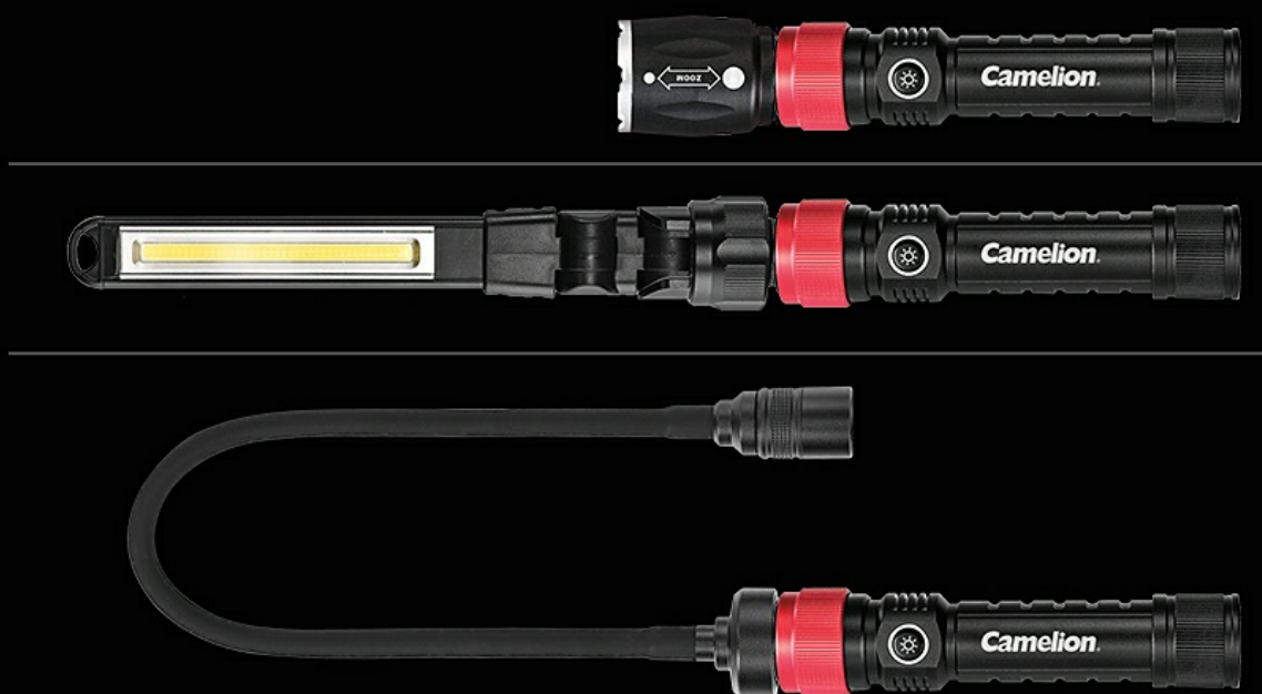
Figure 4: Illustration of the quick-connect system for the three interchangeable light heads: flashlight, work light, and flexible light.
