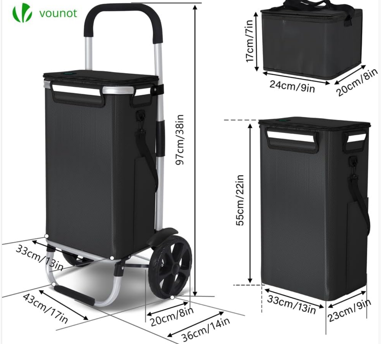
Image: Detailed dimensions of the shopping cart and its insulated bag.
