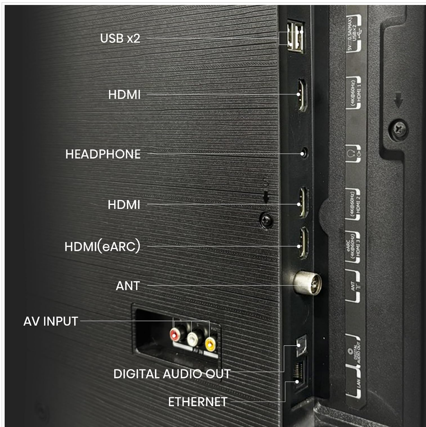
Image: Detailed view of the rear connectivity panel of the TOSHIBA 50C350NP TV, labeling ports such as USB, HDMI, Headphone, AV Input, Digital Audio Out, Ethernet, and ANT (RF).
