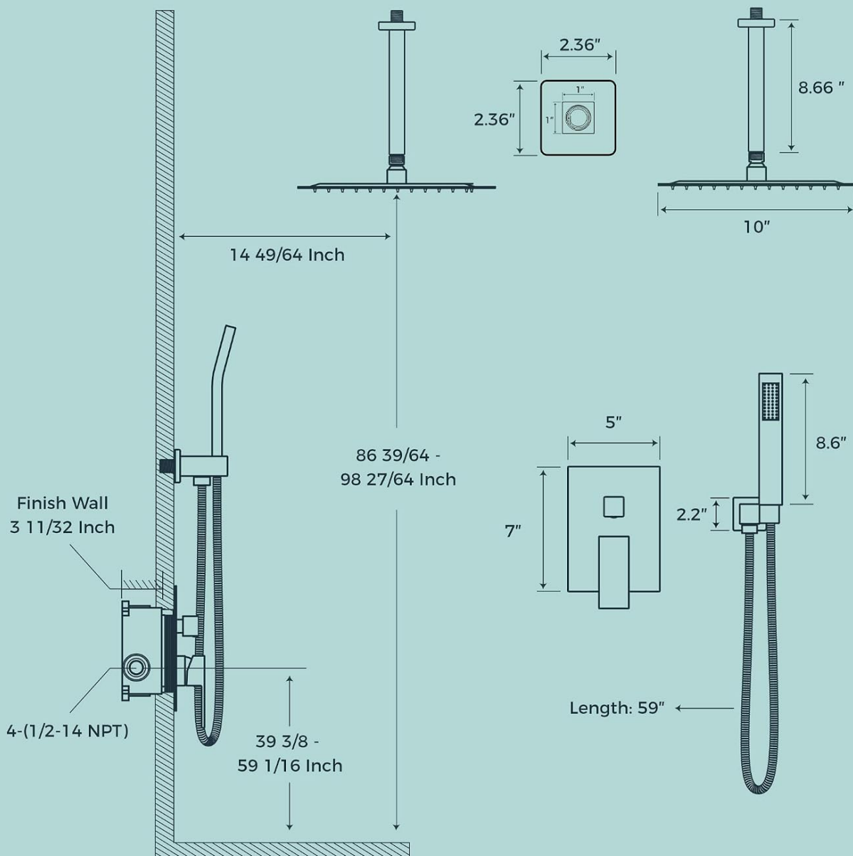
Figure 6: Product size and installation dimensions for planning.
