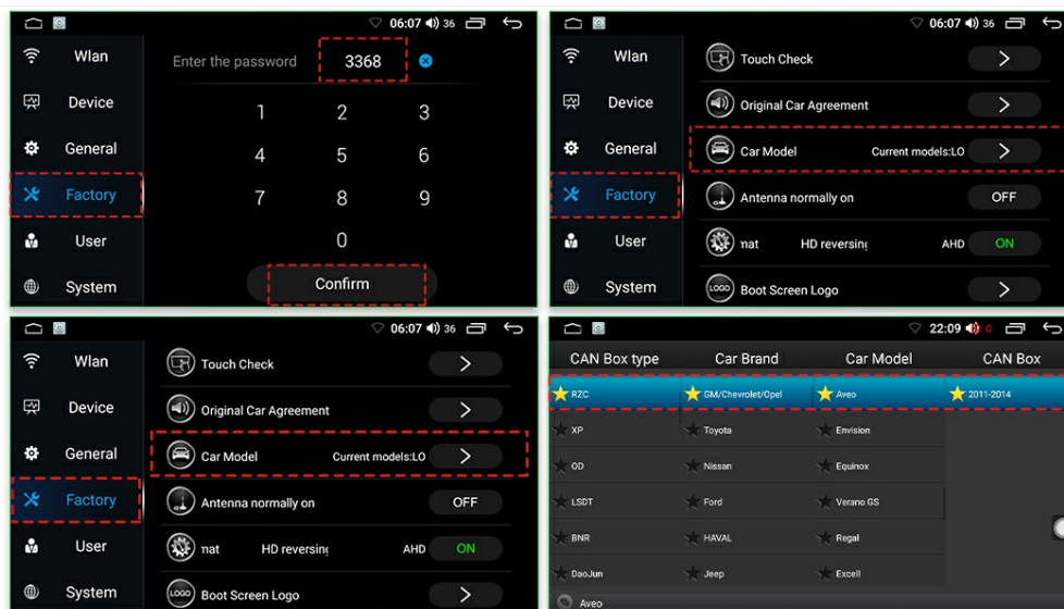
Image 2.3: Car model setting for Chevrolet Sonic to enable steering wheel controls.
