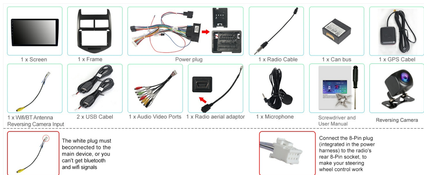
Image 2.1: Included accessories. Ensure all items are present before proceeding with installation.
