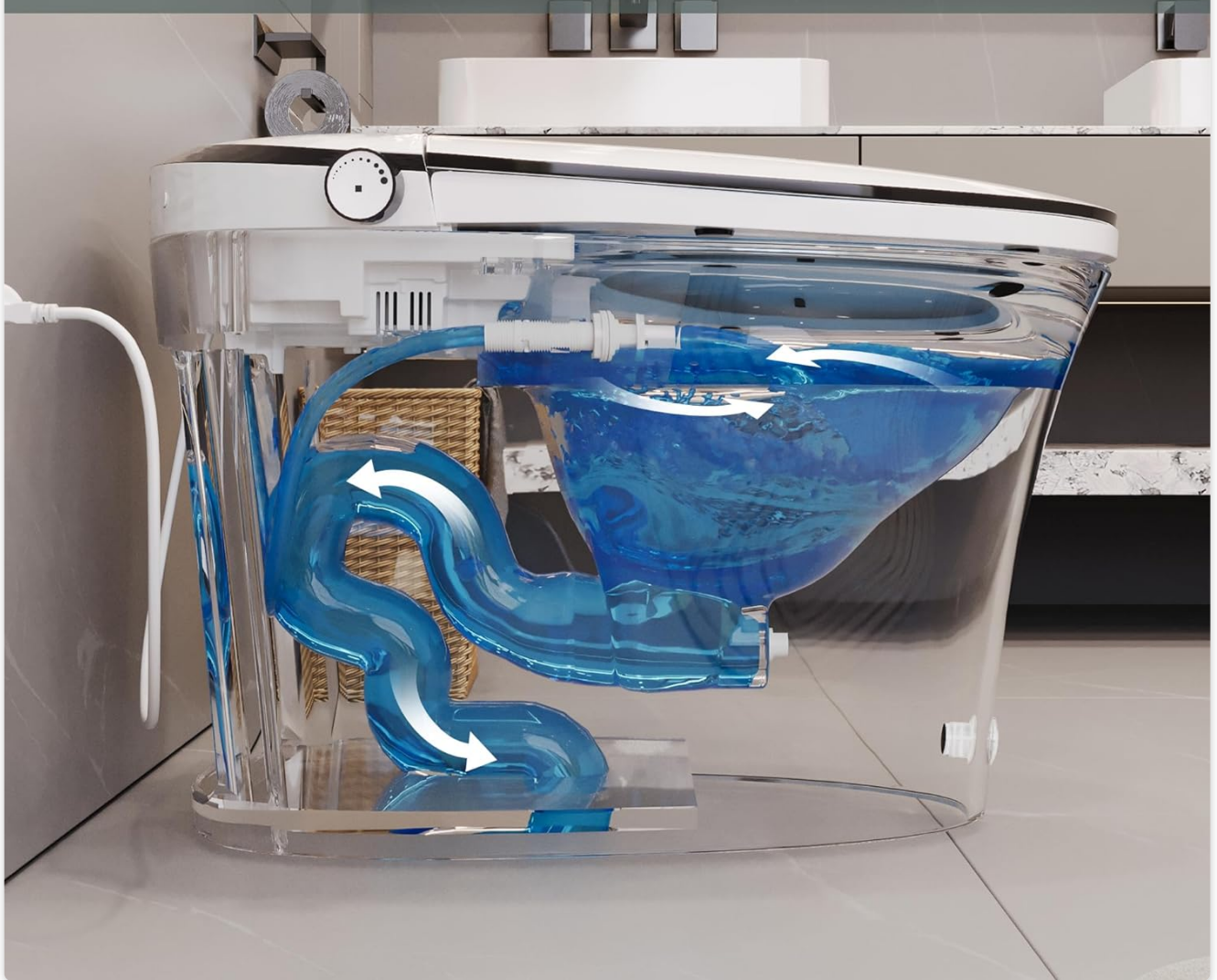
Image 3.5: Illustration of the pre-wetting function, where water coats the bowl surface.
