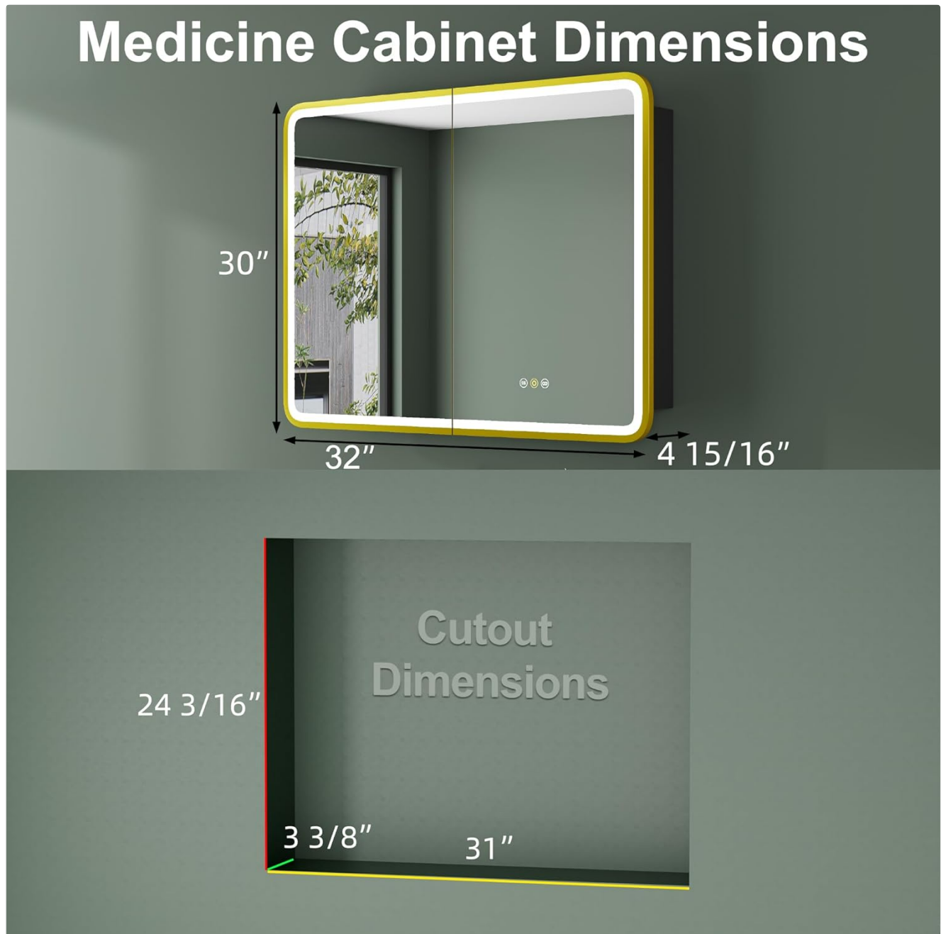
Figure 1: Medicine Cabinet Dimensions and Recessed Cutout Dimensions.
