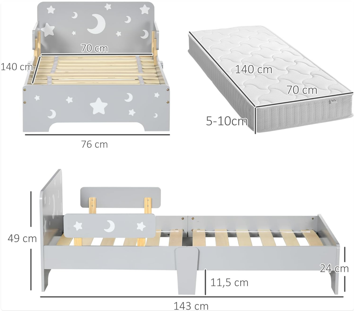
Image 8.1: Product dimensions diagram.
