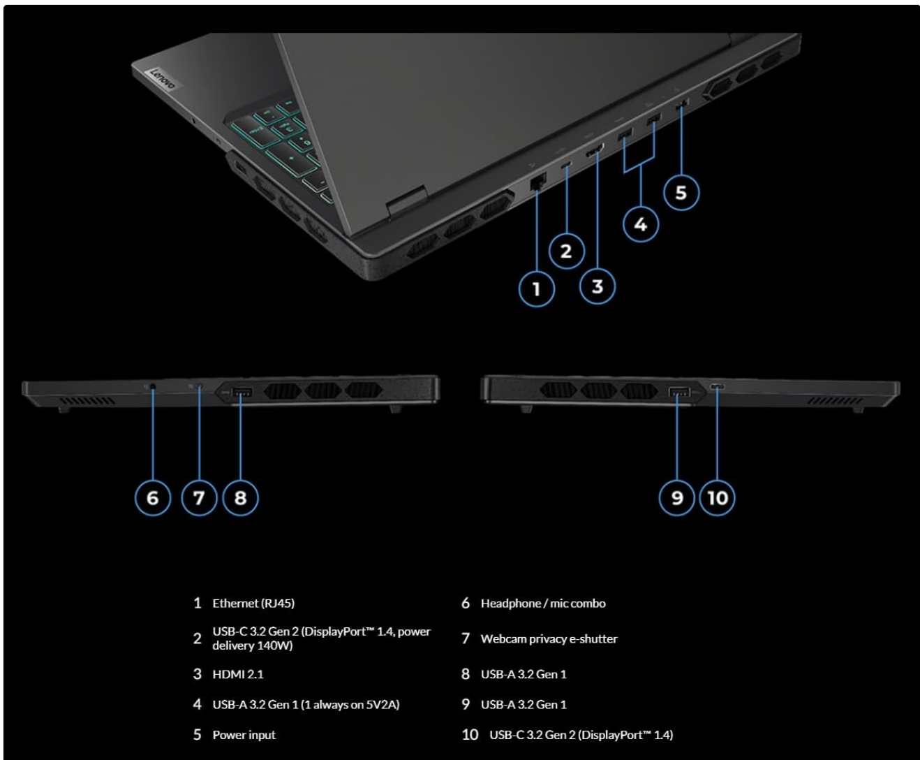
Figure 3: Port layout of the Lenovo Legion Pro 7 Gen 8.
