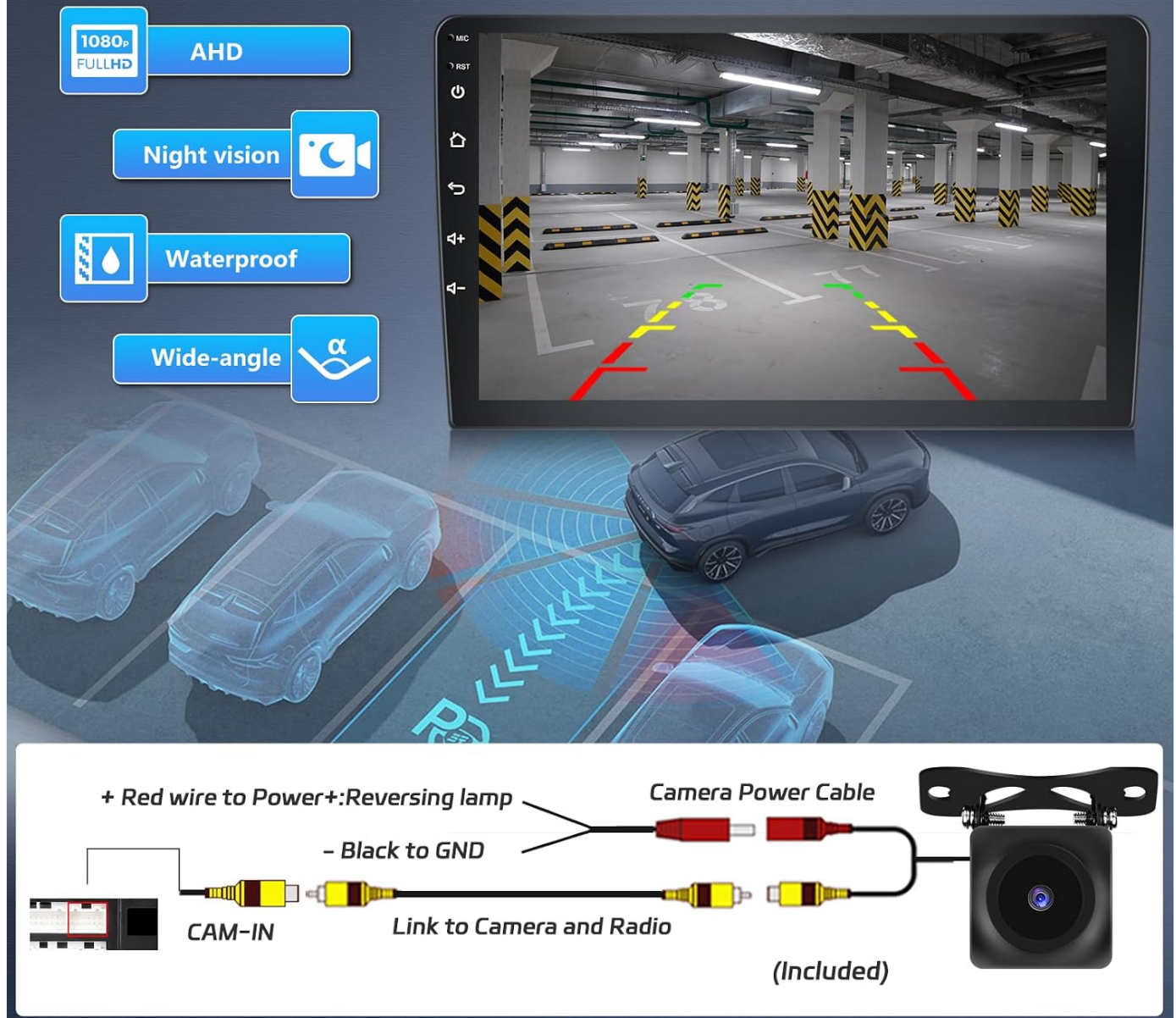
Image 3.1: Backup camera connection diagram and example of the display when reversing.
