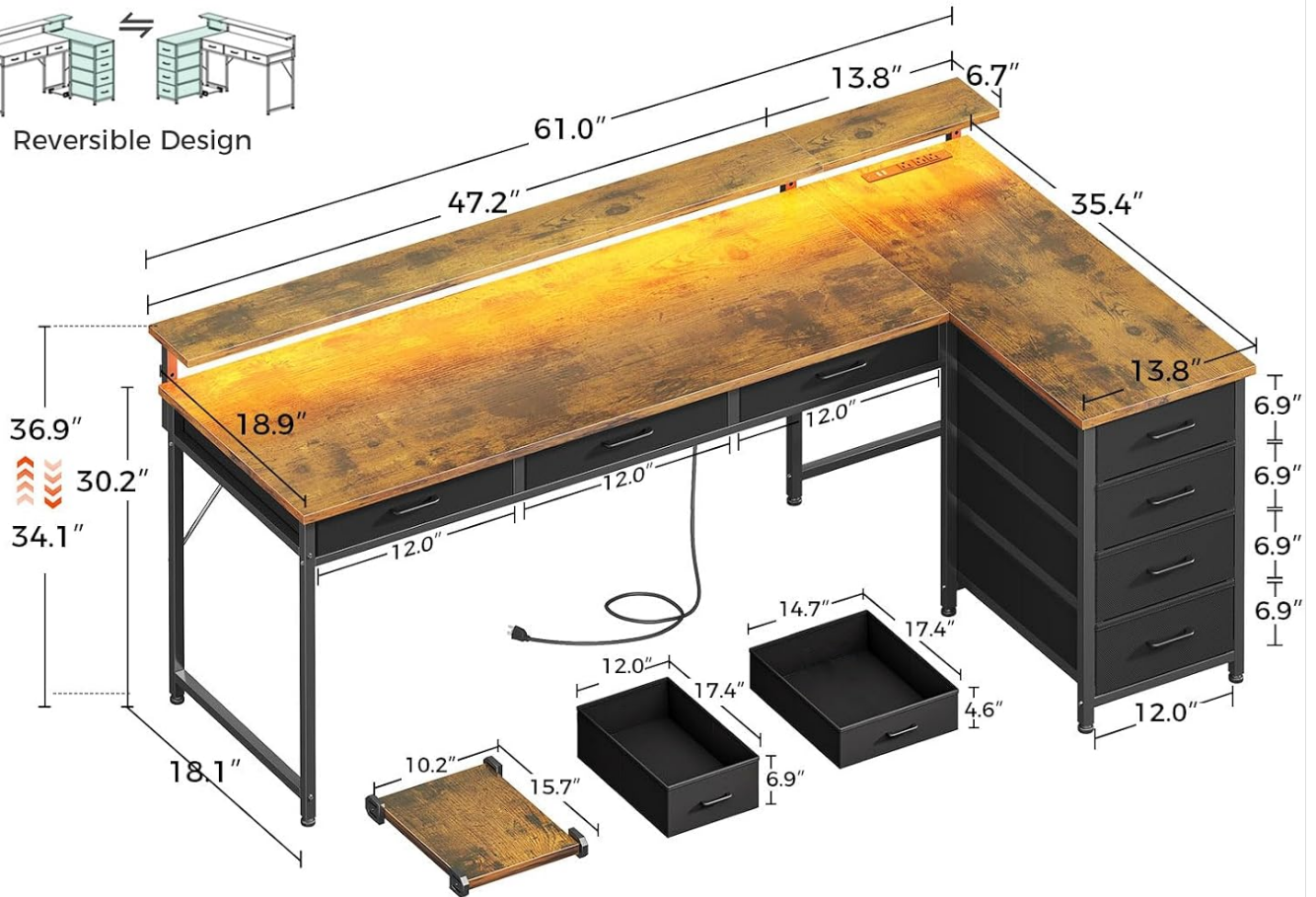
Image: A detailed diagram illustrating the dimensions of the AODK L-Shaped Desk, including overall length, width, height, and specific measurements for the monitor shelf, desk sections, and drawer units.
