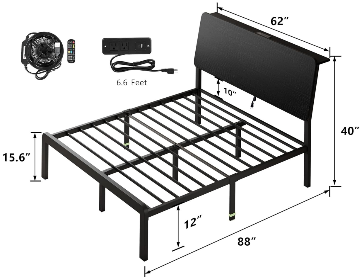
Image: A detailed diagram illustrating the dimensions (length, width, height, under-bed clearance) of the Queen size bed frame.
