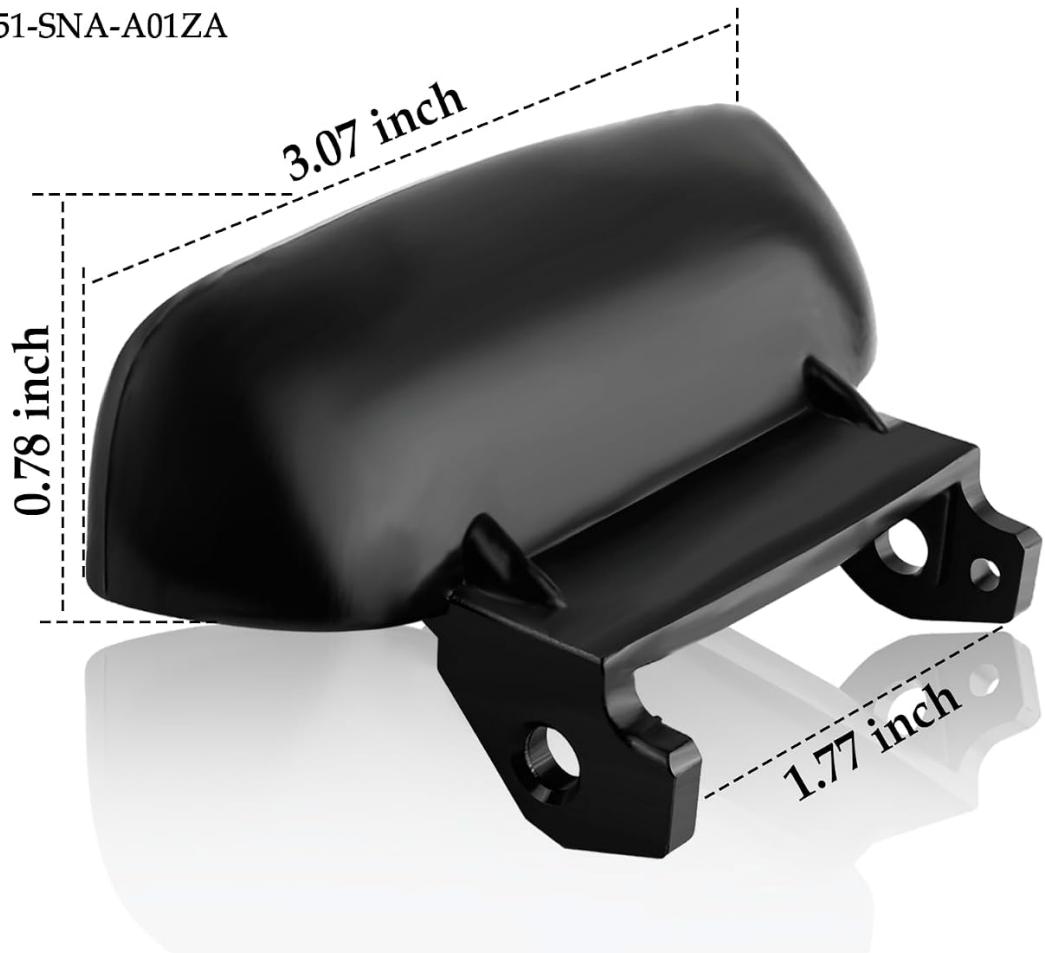
Figure 1: Dimensions of the Center Console Latch. This image illustrates the key dimensions of the replacement center console latch: 3.07 inches in length, 0.78 inches in height, and 1.77 inches in width at the base.
