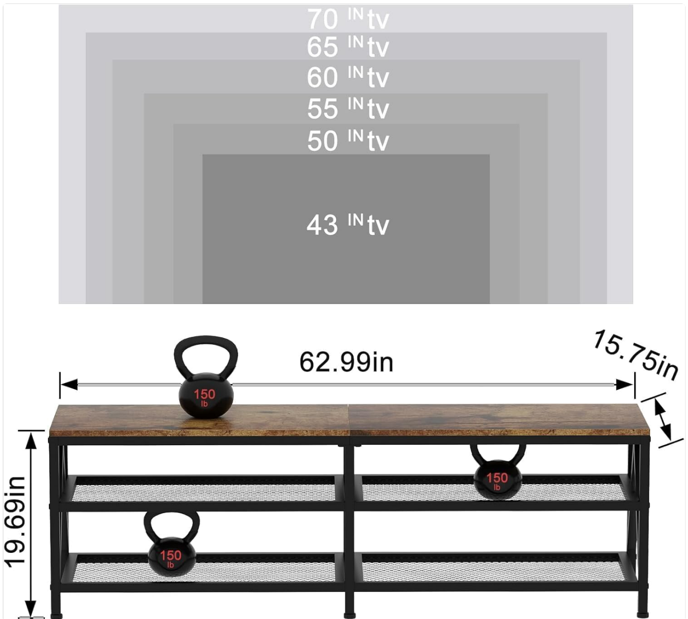
Image 8.1: Dimensional diagram of the TV stand, indicating its overall size and suitability for various television sizes, including up to 70 inches.
