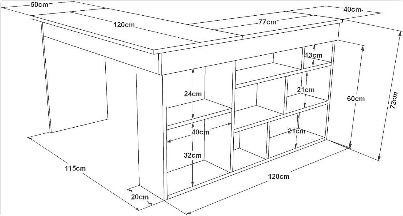
Image 3: Dimensional diagram of the LILEUL Corner Desk, illustrating overall length, depth, height, and internal shelf measurements.
