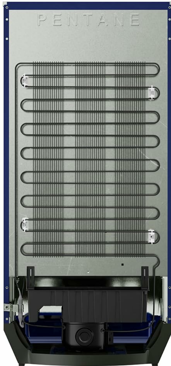
Image: Rear view of the refrigerator, showing the exposed condenser coils and the compressor unit at the bottom.
