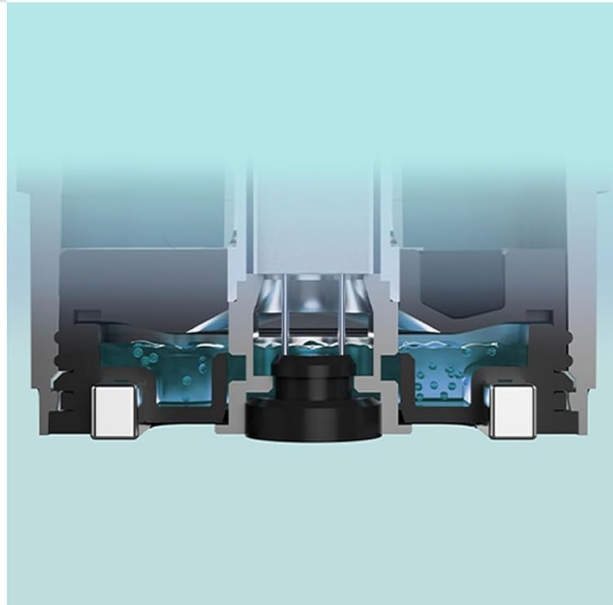
Image 6.1: Illustration of the iCOSM code technology and its leak-proof design.
