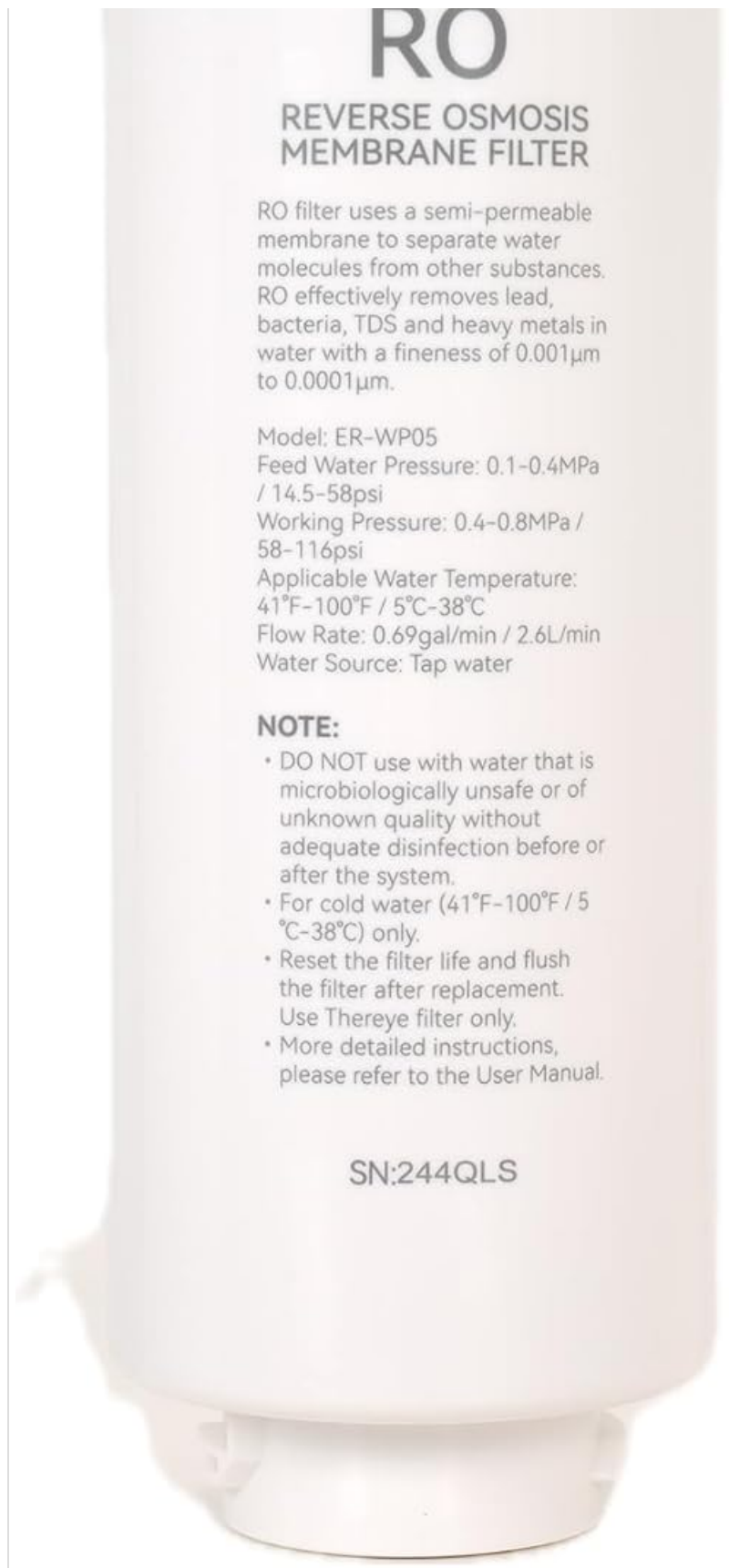
Image 2.1: Thereye RO Water Filter Element WP05.
