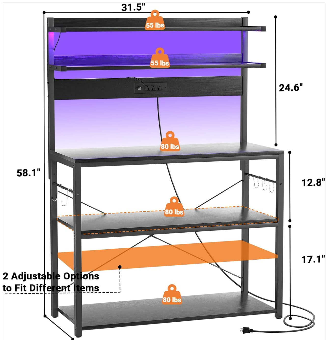
Image: Detailed dimensions and weight capacities for the Aheaplus Bakers Rack.
