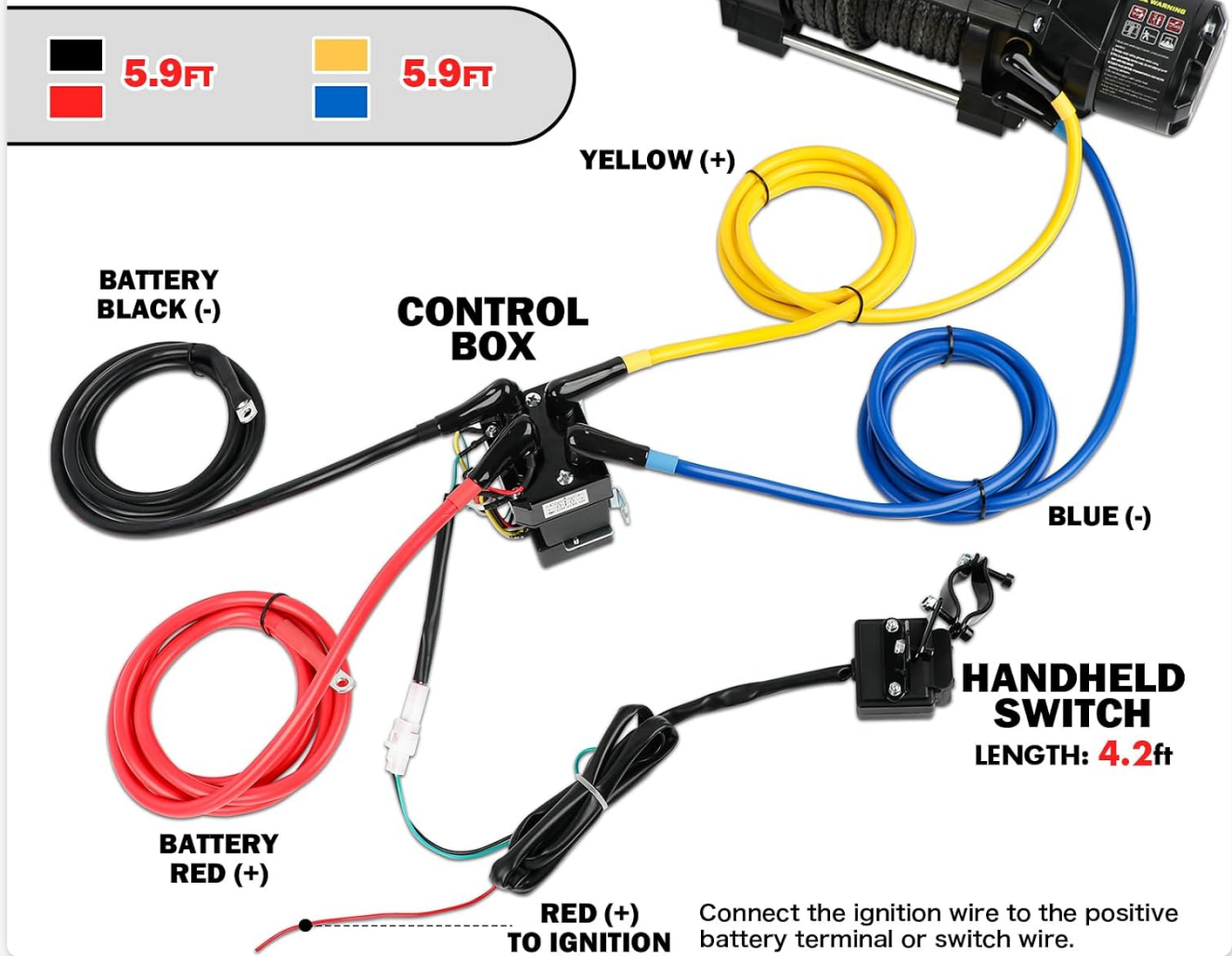
Figure 6: Detailed wiring diagram for the X-BULL Electric Winch.
