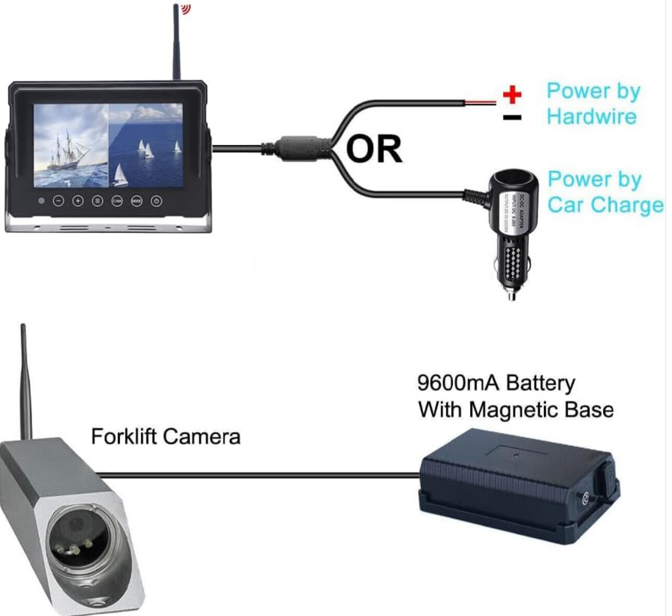
Image: Illustration of the camera and battery bank setup, highlighting the magnetic attachment and power options for the monitor.
