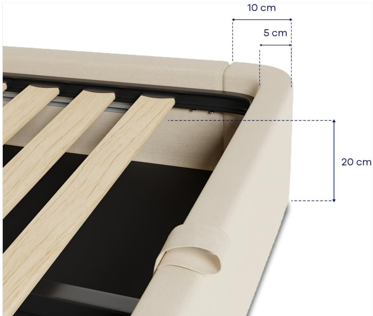
Image 3.2: Detailed view of the bed frame, illustrating slat placement and frame dimensions (e.g., 10 cm, 5 cm, 20 cm depth).
