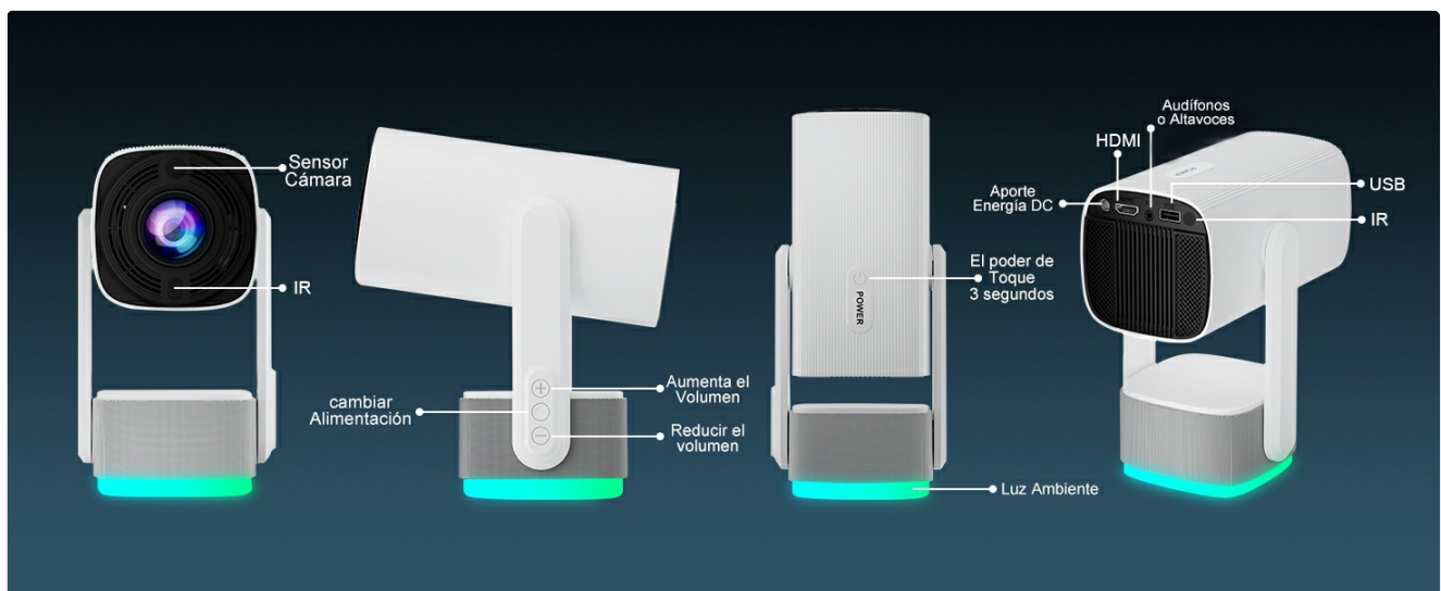
Figure 3.2: Projector Ports and Controls. This diagram illustrates the various input/output ports and control buttons on the Salange K2 projector, including the camera sensor, IR receiver, DC power input, HDMI port, USB port, 3.5mm audio jack, power touch button, volume controls, and ambient light.
