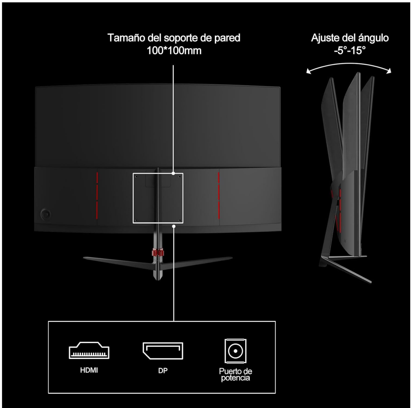
Image: Rear view of the monitor illustrating port locations (HDMI, DP, Power), VESA mount compatibility, and tilt adjustment range (-5° to 15°).
