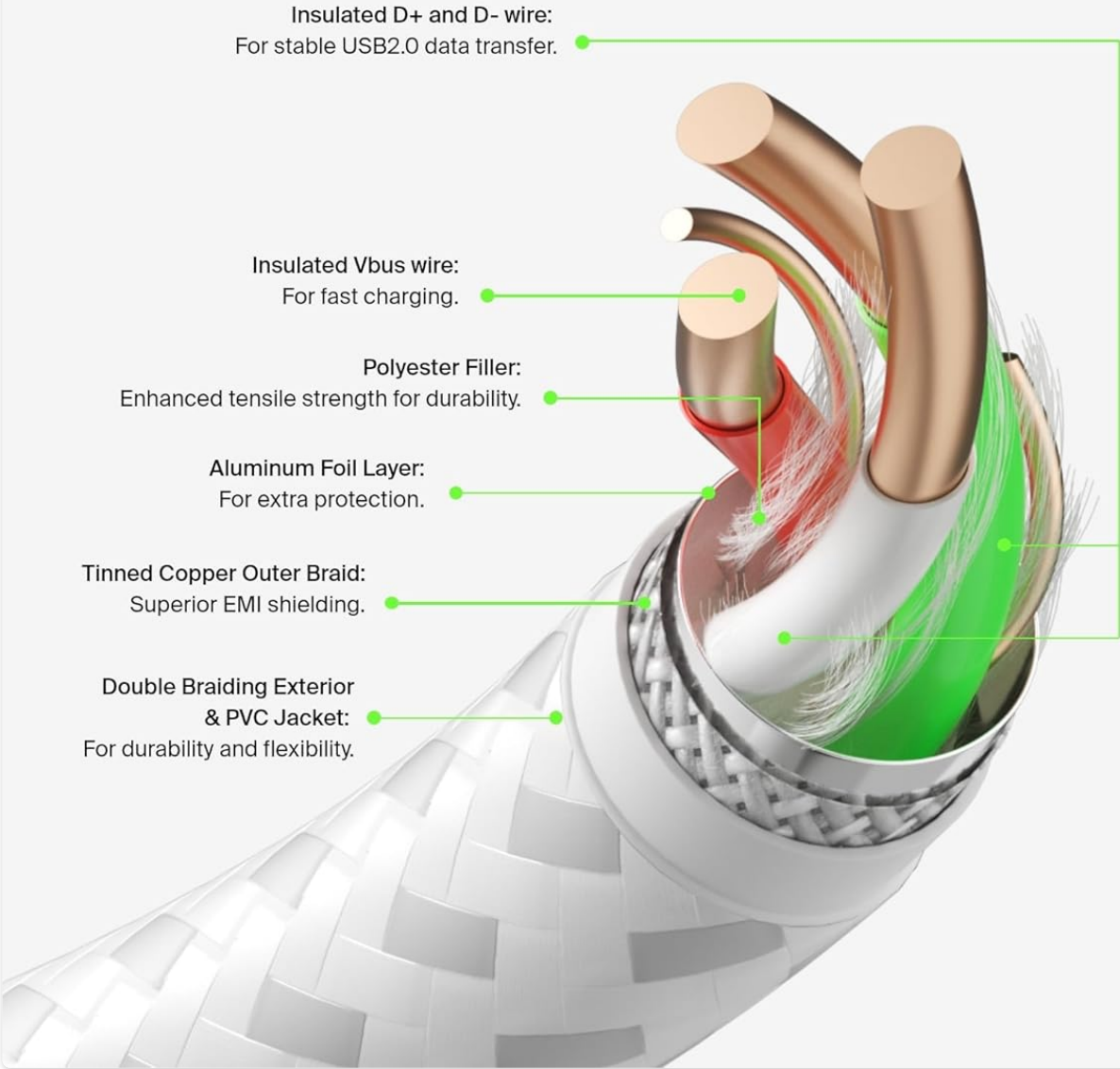
Image: An exploded view diagram illustrating the engineered layers of the cable, including insulated wires, polyester filler, aluminum foil, tinned copper braid, and double braiding for safety and durability.
