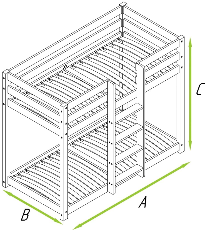
Image: Technical diagram illustrating the dimensions of the ADEKO CLPN bunk bed, including length, width, and height, along with the recommended mattress size of 70x140 cm.
