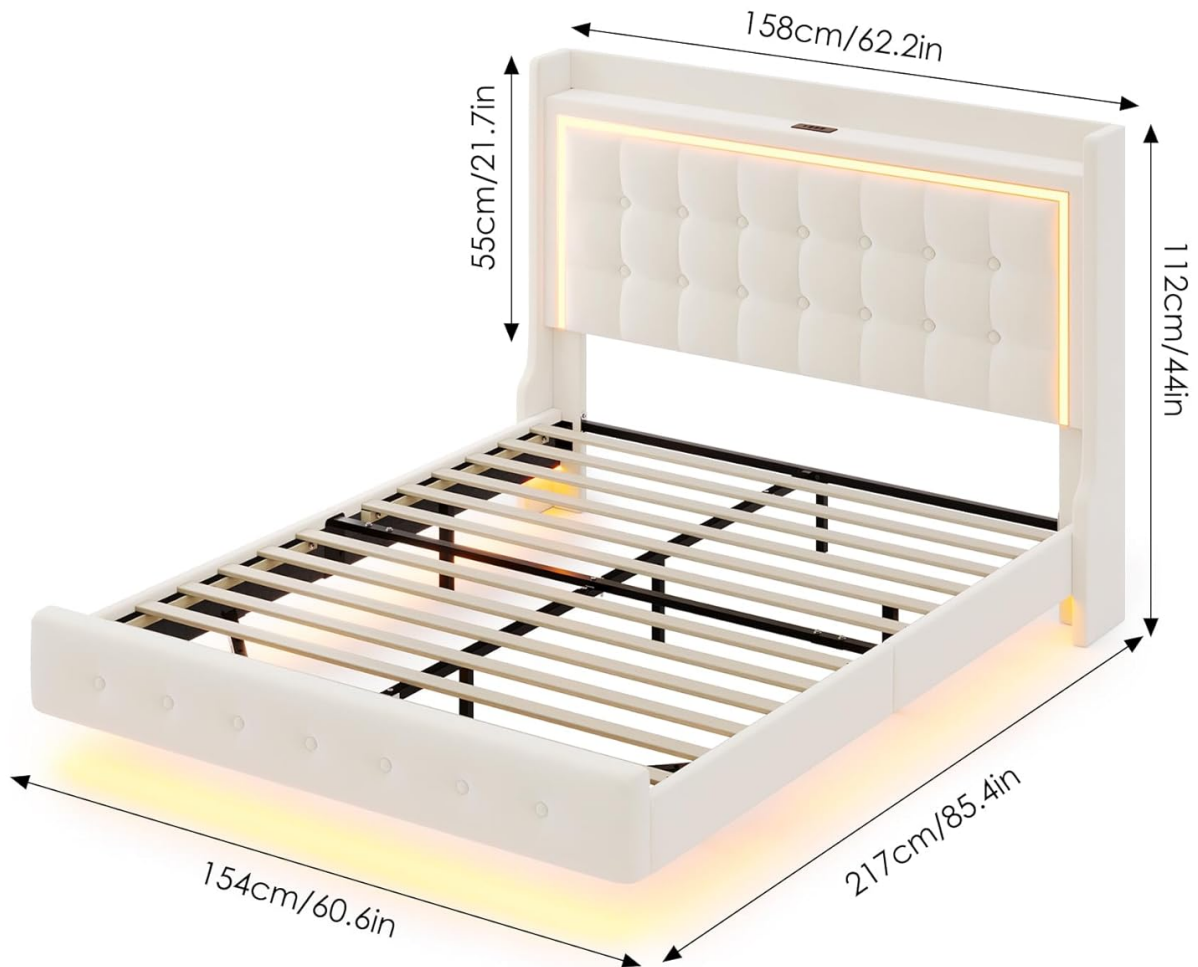
Image: Detailed dimensions of the Queen size bed frame.
