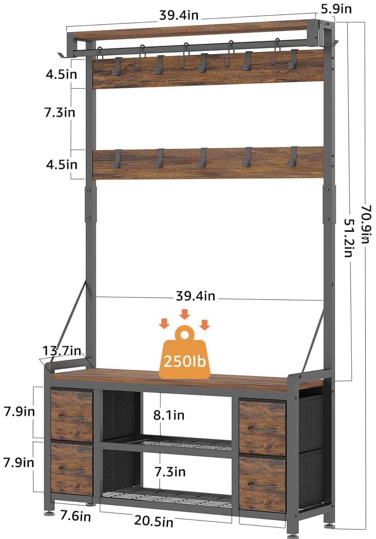
Image: Detailed diagram illustrating the dimensions of the hall tree, including height, width, and depth of various sections.
