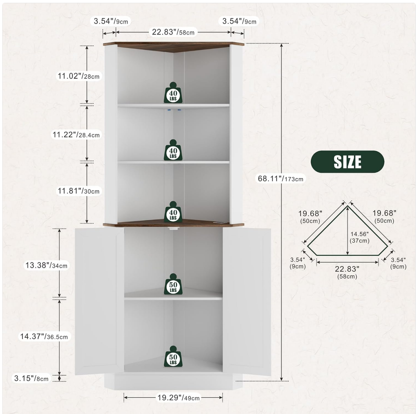
Figure 4.1: Cabinet dimensions and internal shelf layout. This diagram provides an overview of the cabinet's size and the arrangement of its shelves.
