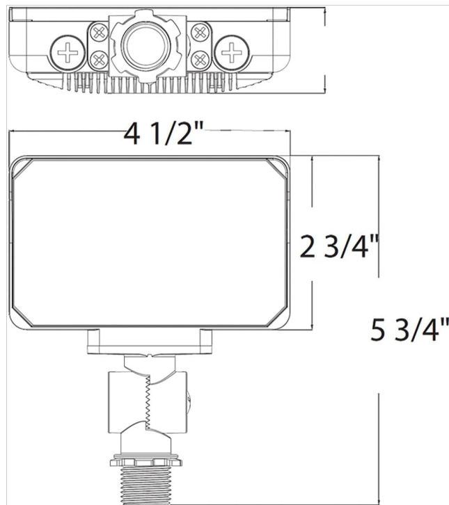
Figure 2: RAB X34 Series LED Flood Light Dimensional Drawing. This diagram provides key measurements for the fixture, including length, width, and height, useful for installation planning.
